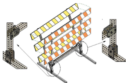
Part #: TBB3A-Z Collapsible barricade assembly - two plates & required hardware to connect one upright to one foot 10 sets/box
